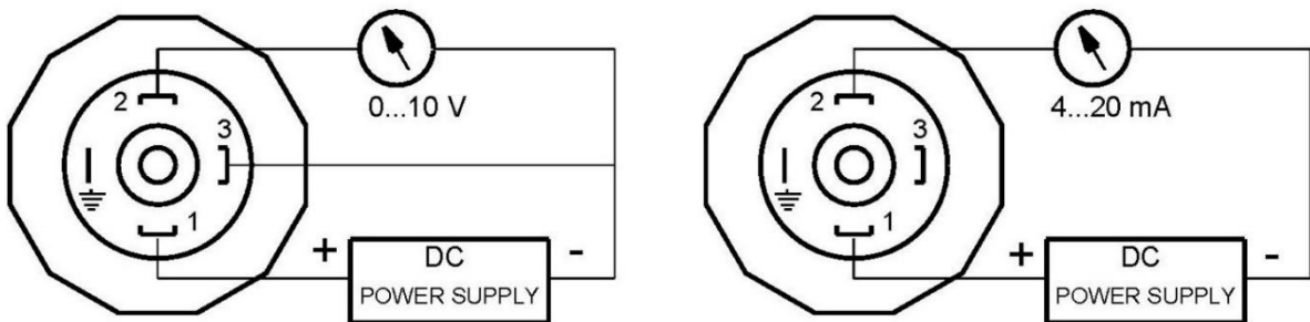
Figure 1. Transmitter connector diagram
