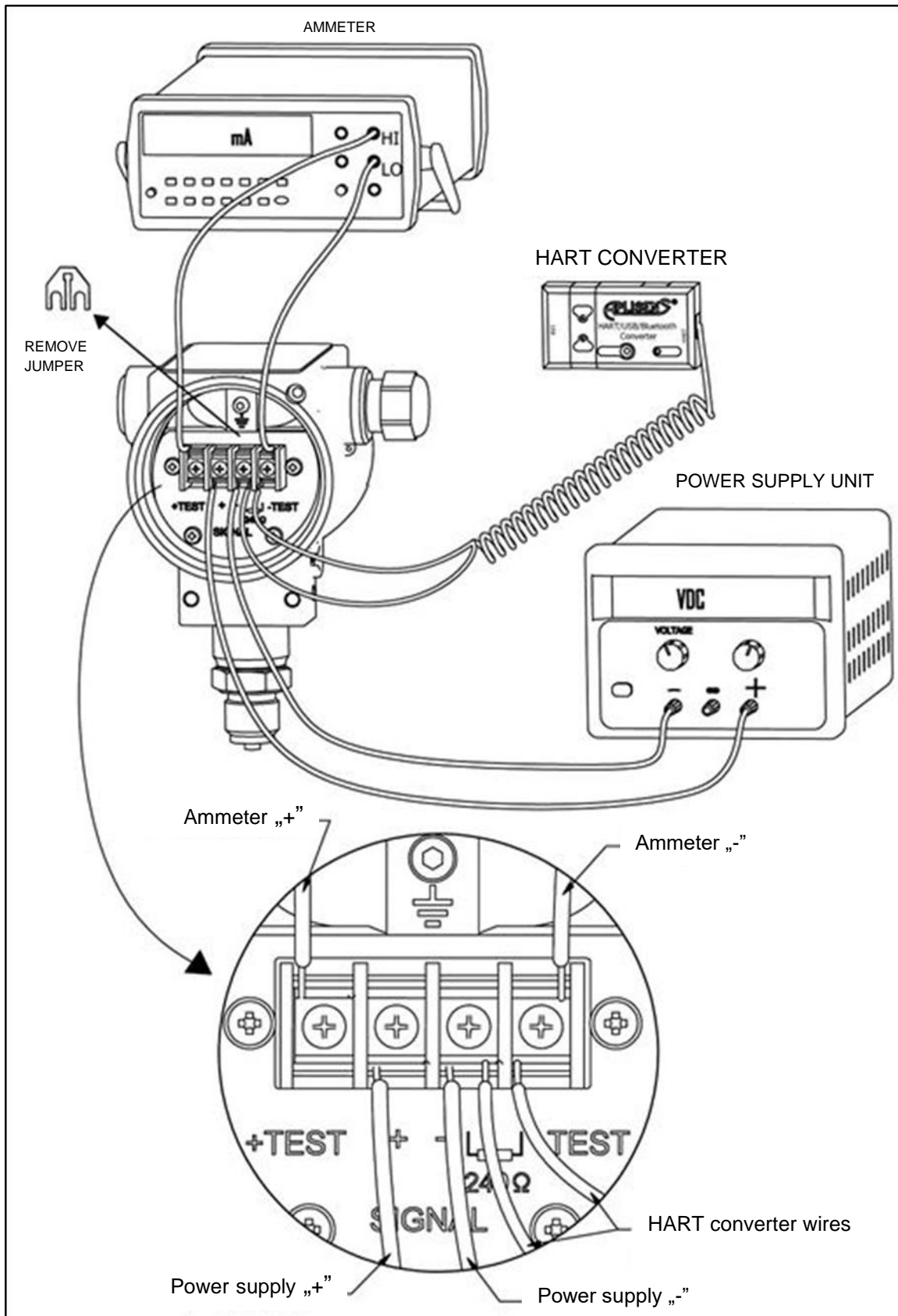
Fig. 1. Transmitter connection to the current loop for verification testing
